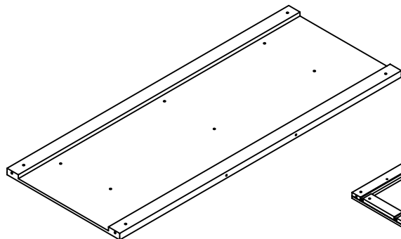
A TOP Panel superior DESSUS T9302096010
